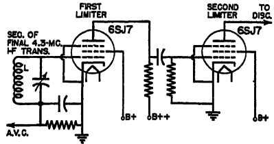
Circuit diagram of a two-tube cascade limiter for a frequency-modulated receiver.
